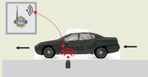
WRS-2010 Wireless Roadway Sensor
